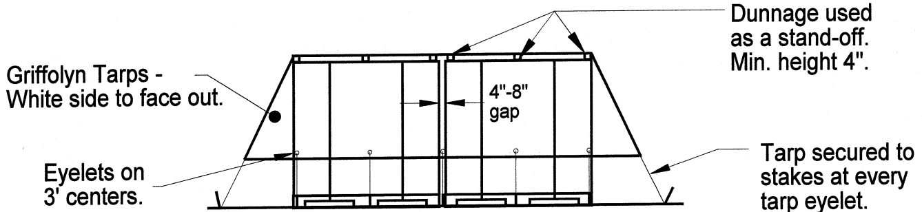
Front Elevation - Typical Double Row
